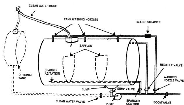
SPRAY TANK NOZZLE SYSTEM
